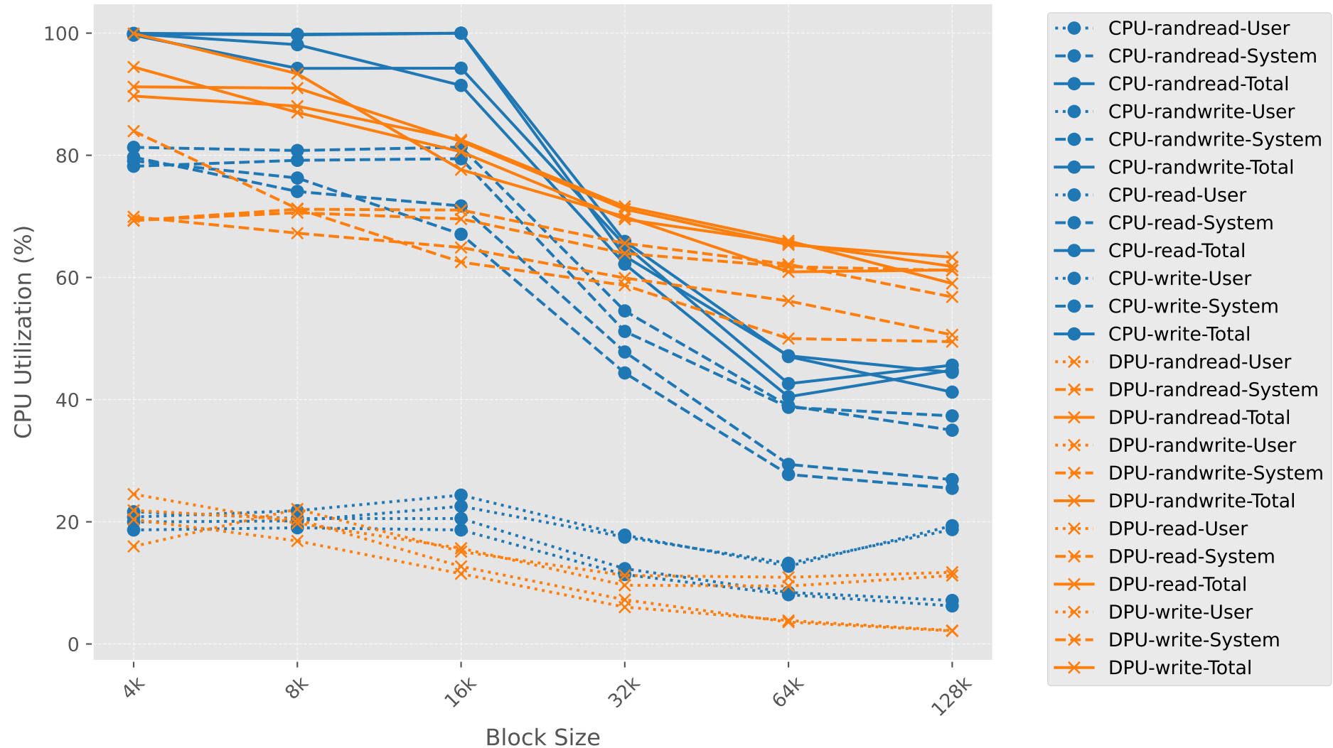
CPU Total vs Block Size
